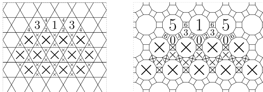
Figure 2: The order in which faces in the next row become infected, when proving that the lattice (3.6.3.6) has threshold 2 and that the lattice (4.6.12) has threshold 3.
