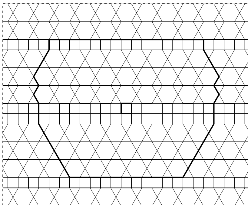
Figure 5: A tiling in \mathcal{T}_{strips} , along with a marked face and \mathcal{A}_4 .
