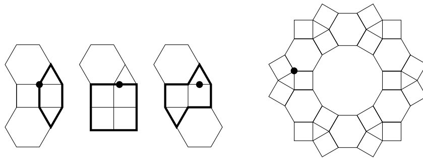
Figure 4: Left: The three possibilities for C when T contains a vertex of type 3.4.4.6. Right: A configuration, C , of 31 faces in which each face has at most two neighbors outside C .
