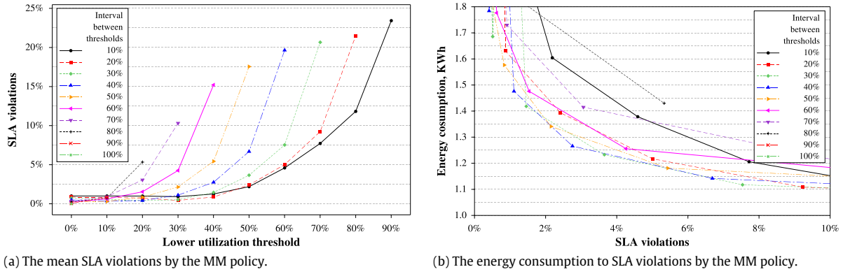
Fig. 4. The energy consumption and SLA violation analysis for the MM policy.
