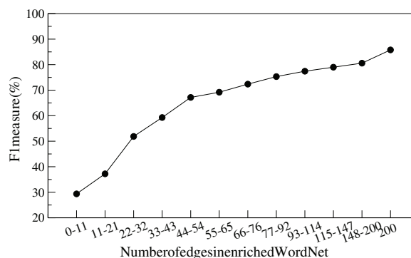
Figure 3: Performance of KPP by number of edges.
