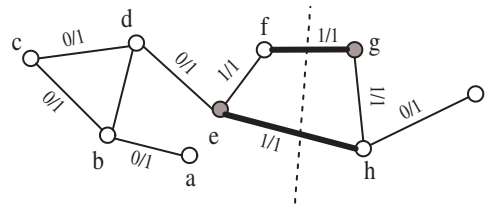
Figure 2: The maximum flow between nodes e and g (edges are labeled with the pair flow/capacity).
