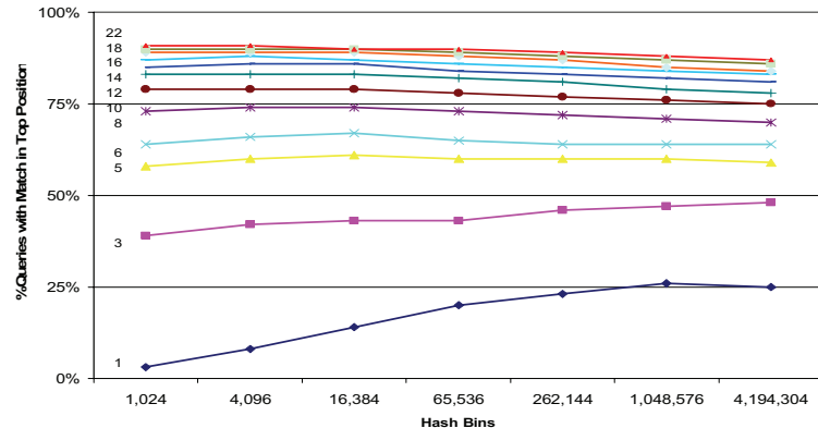
B. Match in Top Position Shown for System with l=1-22 Sets of Hashes
