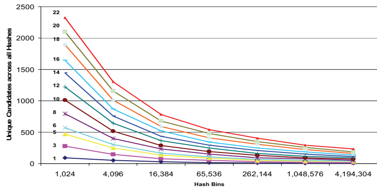
A. Unique Candidates Across All Hashes Shown for System with l=1-22 Sets of Hashes
