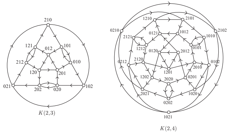
Figure 1: The Kautz digraphs K(2,3) and K(2,4) .
