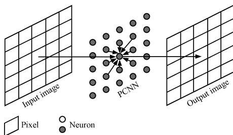
Fig. 3 Connection model of PCNN neuron
