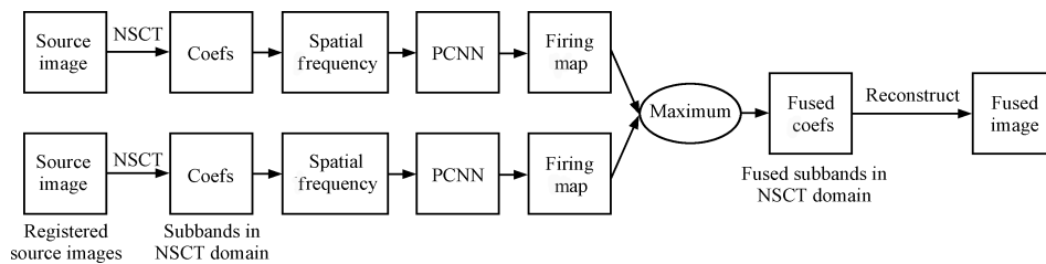
Fig. 5 Schematic diagram of NSCT-SF-PCNN fusion algorithm
