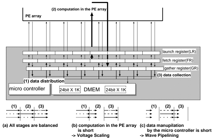
Figure 2: Operations of the microcontroller of CMA-1
