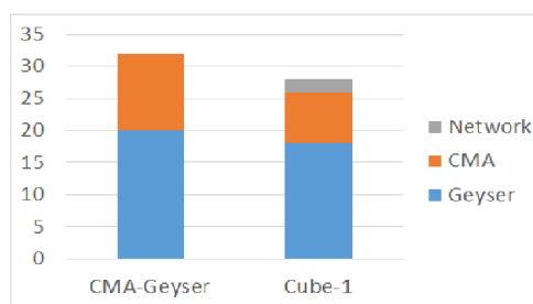
Figure 11: Power Consumption of JPEG Decoder Execution
