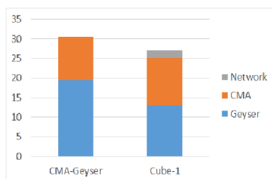
Figure 10: Power Consumption of Gray Scale Execution
