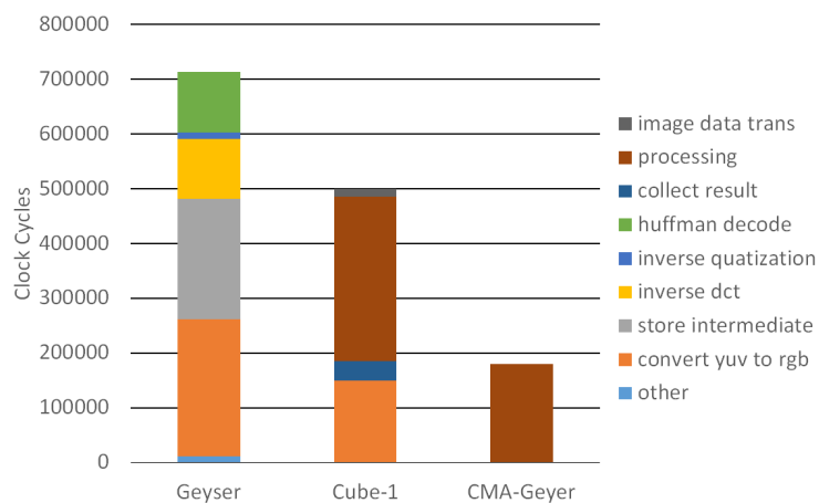
Figure 9: Execution cycles of JPEG decoder
