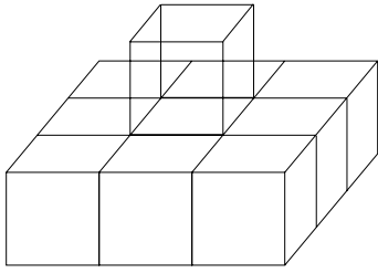
Figure 3: A polytope which can be tiled by 3d -dominoes but all of whose sides are odd.
