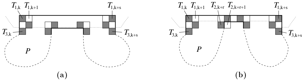
Figure 5: Two subcases in the proof of Lemma 2.2.
