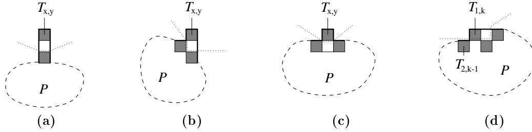
Figure 4: The four cases considered in the proof of Lemma 2.2.
