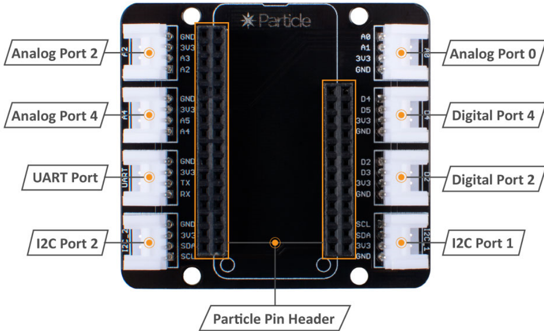
Figure 1. hardware overview
