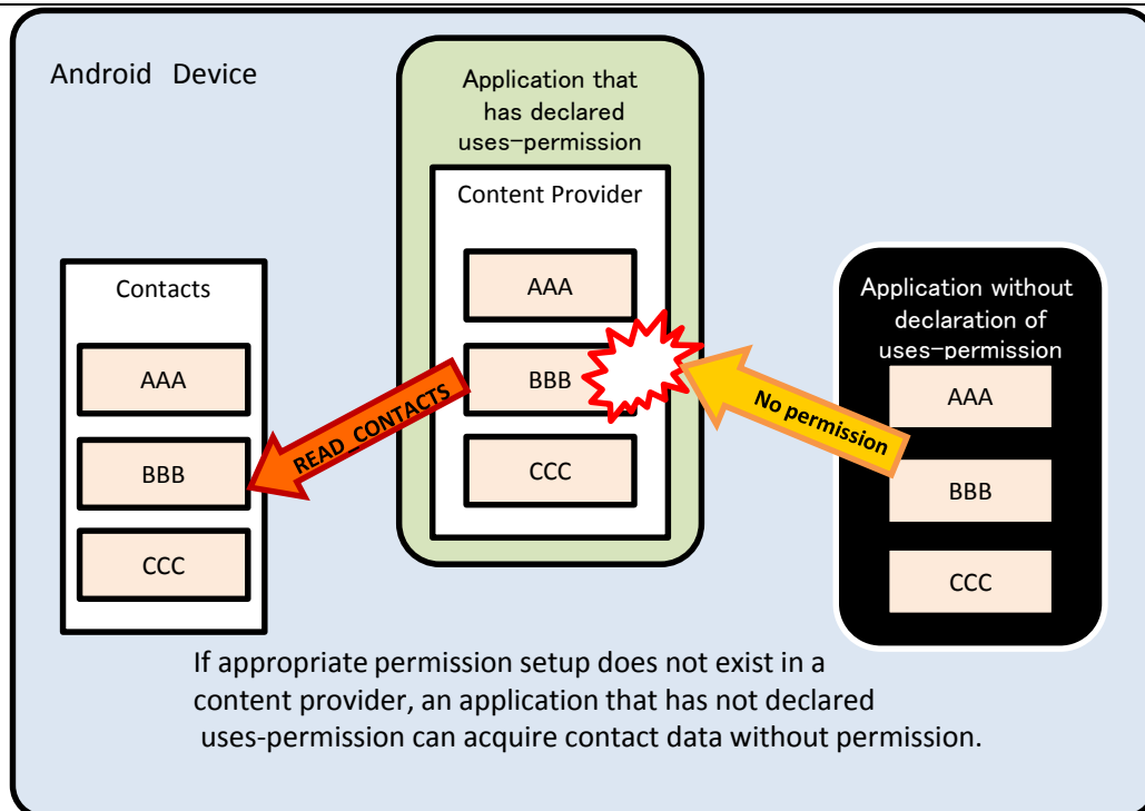
Figure 5.2–9 An Application without Permission Acquires Contacts
