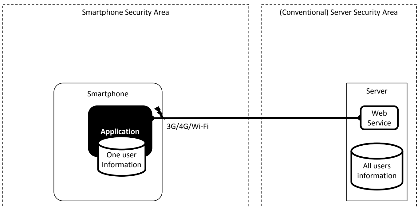
Figure 3.1-3 Typical Environment an Android Application Behaves in
