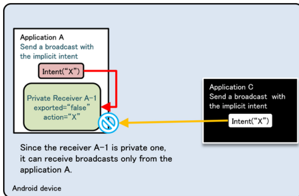
Fig. 4.2.4: An Example of Normal Behavior
