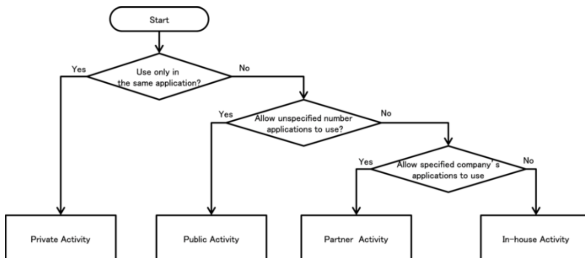
Fig. 4.1.1: Flow Figure to select Activity Type
