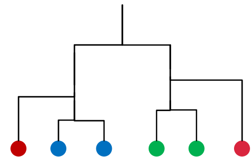
Dendrogram
