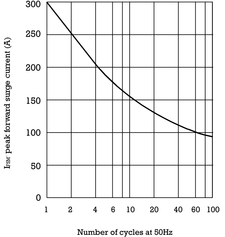
MAXIMUM NON-REPETITIVE PEAK FORWARD SURGE CURRENT
