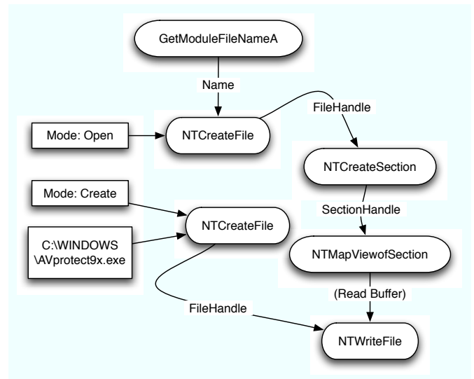
Figure 1: Partial behavior graph for Netsky.
