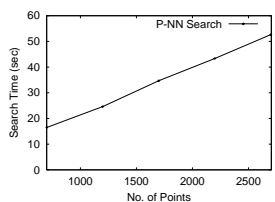
Figure 10: Search Time (Synthetic Data)
