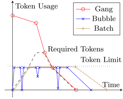
Figure 14: Resource utilization during query execution
