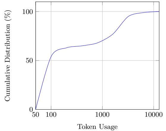
Figure 8: Cumulative token distribution from production cluster
