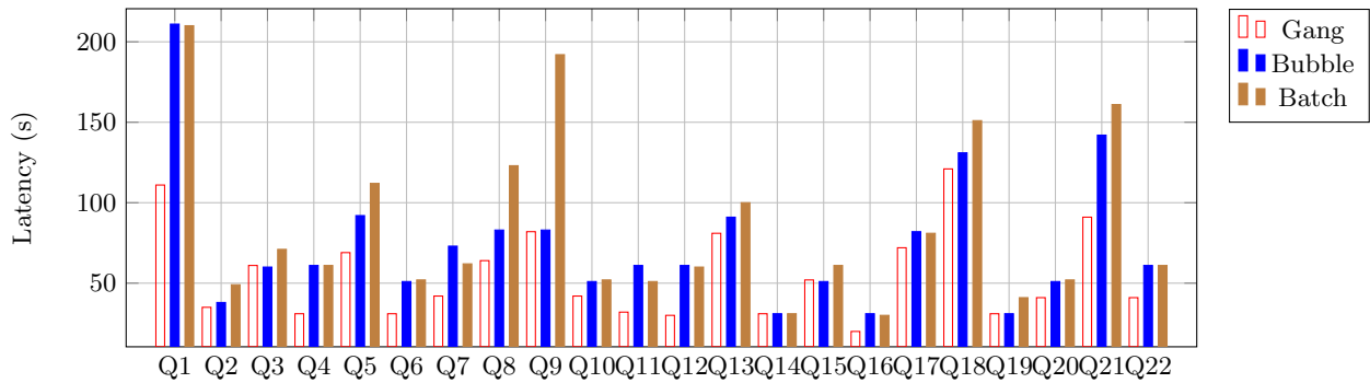
Figure 9: Performance comparison among different execution models
