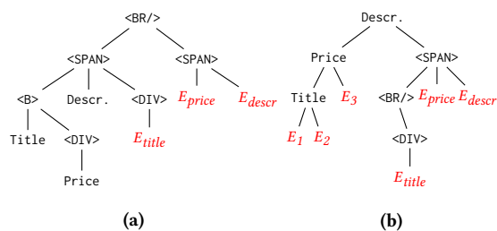
Figure 2: Landmark-trees for the running example
