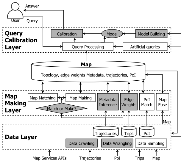
Figure 1: QARTA Architecture
