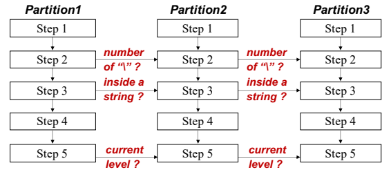
Figure 4: Dependences in Index Construction.
