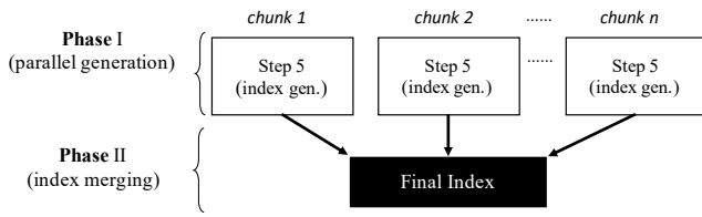
Figure 8: Two-Phase Index Construction.
