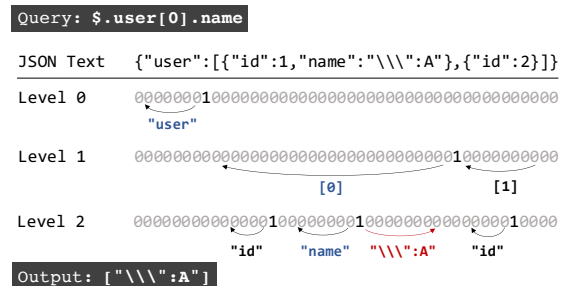
Figure 3: Querying via Structural Indices.
