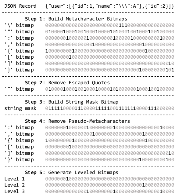
Figure 2: Example Structural Index Construction.
