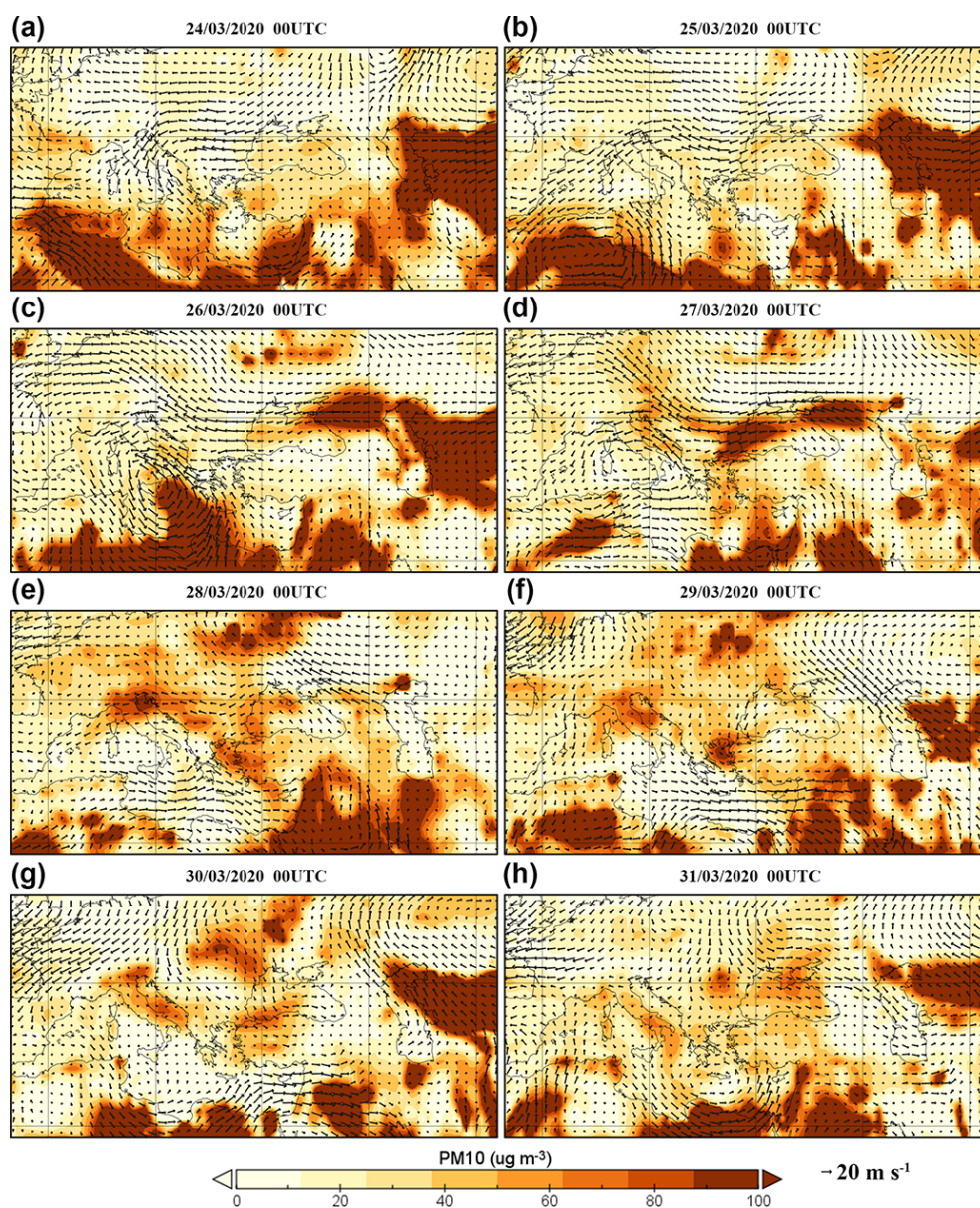
Figure 2. Maps of the PM 10 (colors, in µg m -3 ) and horizontal surface wind (arrows) relative to each day in the period from 24 to 31 March at 00:00 UTC (a–h). The maps were created with Panoply starting from ERA5 reanalysis. Panels (a) to (h) refer to the respective days from 24 to 31 March 2020.
