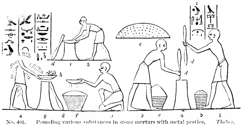
a, a, i, mortars. d d, pestles. Figs. 1 and 2 are alternately raising and letting fall the pestles into the mortar. Figs. 3 and 4 are sifting the substance after it is pounded; the coarser parts, h, being returned into the mortar to be again pounded. The inscriptions are the directions: k reads, 'Hasten all the work in taking care of all that is given out; make ye the bread'; l, 'The pounding of the corn in the storehouses of . . .'
