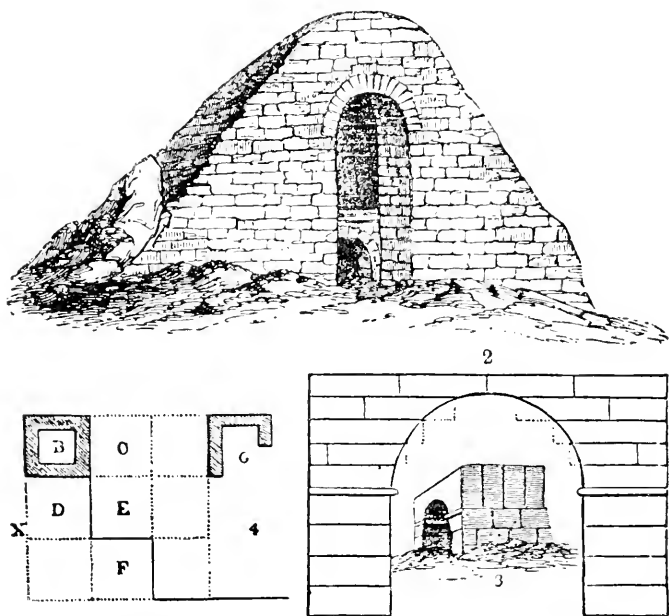
No. 427. Fig. 1. Vaulted rooms and doorway of a rude brick pyramid at Thebes. 2. An imitation of an arch at Thebes. 3. Another at Abydus. 4. Mode of commencing a quarry.
