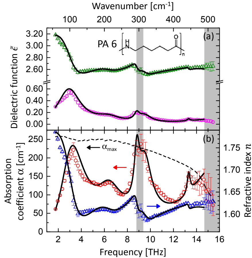
Fig. 6. PA6: (a) Real (green) and imaginary (magenta) part of the dielectric function. Black lines are fits based on six Lorentzian modes. (b) Absorption coefficient (red-left ordinate axis) and refractive index (blue-right ordinate axis). Black solid lines are the re-calculated index and absorption coefficient. Dashed black line is the maximum absorption that can be reliably measured by our spectrometer (left ordinate axis).
