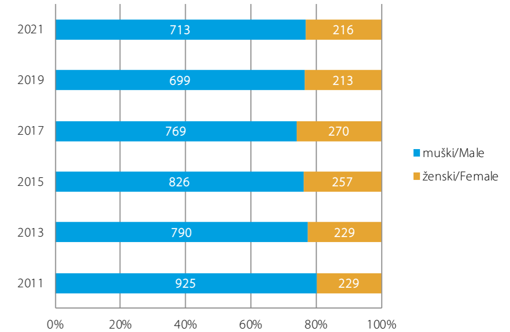
Grafikon 11. Nasilne smrti prema spolu Graph 11. Violent deaths by sex
