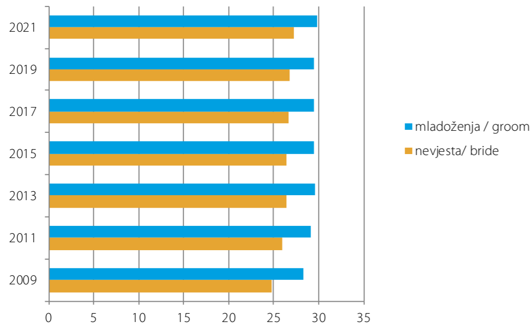
Grafikon 15. Prosječna starost – prvi brak Graph 15. Average age – first marriage
