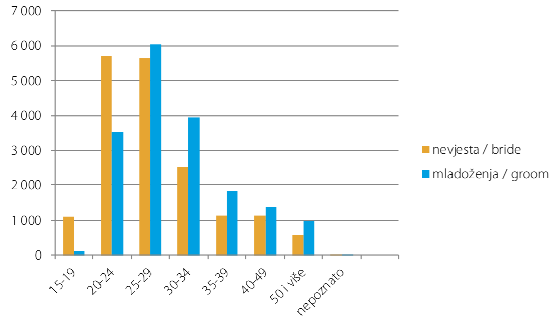
Grafikon 14. Sklopljeni brakovi prema starosnoj grupi nevjeste i mladoženje u 2021. Graph 14. Marriage by age group of bride and groom in 2021
