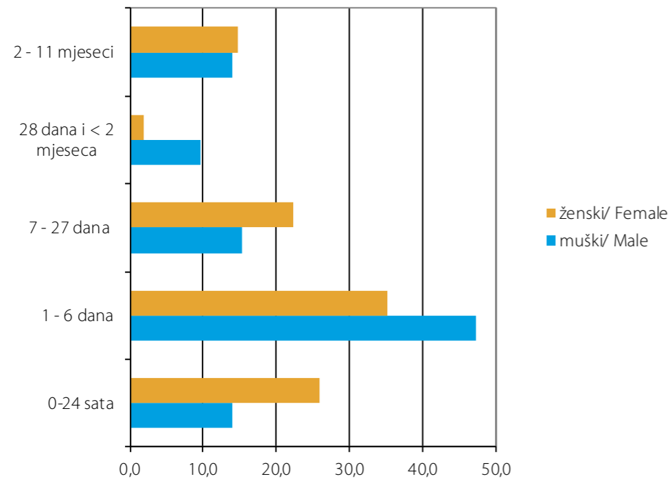
Grafikon 10. Struktura umrle dojenčadi po starosti i spolu u 2021. Graph 10. Distribution % — Infant deaths by age and sex in 2021
