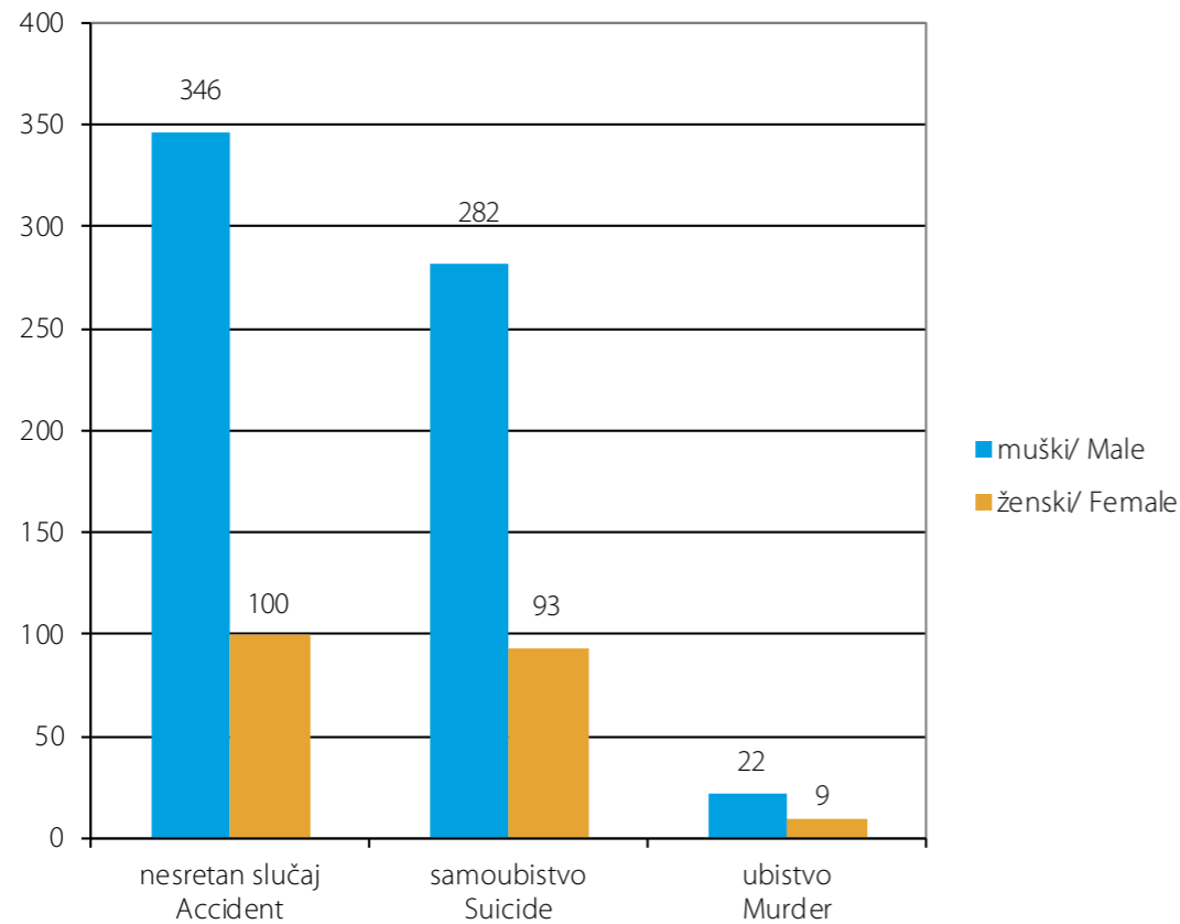
Grafikon 13. Nasilne smrti prema vrsti i spolu u 2021. Graph 13. Violent deaths by type and sex, 2021
