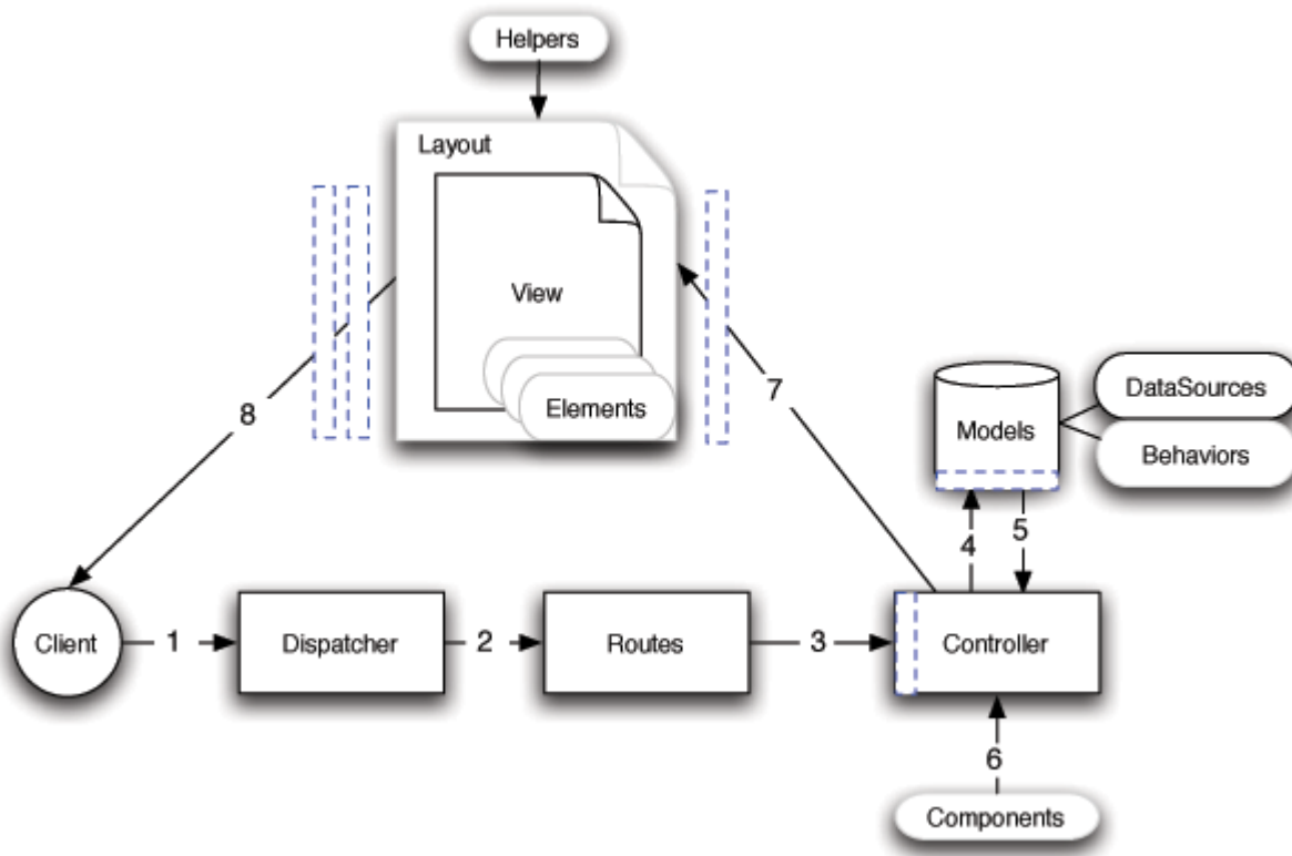
Fig. 1: Flow diagram showing a typical CakePHP request
