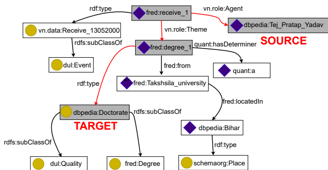
Figure 1: Schematic example of our approach. The RDF graphlet generated by a machine-reading tool (FRED) for the claim “Tej Pratap Yadav receives a doctorate degree from Takshila University in Bihar” (a known misinformation claim [26]). The shortest undirected path between the source (dbpedia:Tej_Pratap_Yadav) and target (dbpedia:Doctorate) is shown in red. The nodes along the path are highlighted in gray.
