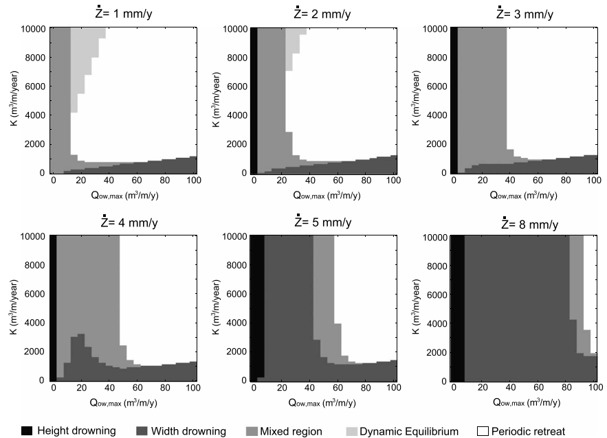
Figure 11. Regime diagrams as a function of the maximum overwash flux Q_{ow,max} and the shoreface flux constant K for different values of the sea-level rise rate z . The back-barrier lagoon slope is \beta = 0.001 . The other parameter values are included in Table 3.
