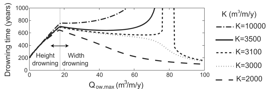
Figure 15. Time of drowning during barrier landward migration as a function of the maximum overwash Q_{OW,max} . Input parameter values are included in Table 3.
