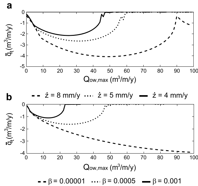
Figure 14. Average sediment loss to the shoreface toe as the barrier migrates landward (i.e., \bar{q}_t < 0 ) as a function of the maximum overwash flux Q_{OW,max} for different (a) sea-level rise rates \dot{z} and (b) back-barrier lagoon slopes \beta . Figure 14a includes three transects of three regime diagrams from Figure 11 for K=2000 \text{ m}^2/\text{y} , and Figure 14b includes three transects of regime diagrams from Figure 12 for K=4000 \text{ m}^2/\text{y} .
