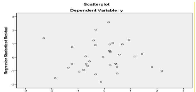
Fig. 2. Multicolinearity test.
