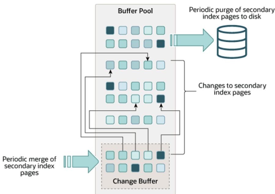
Figure 14.3 Change Buffer
