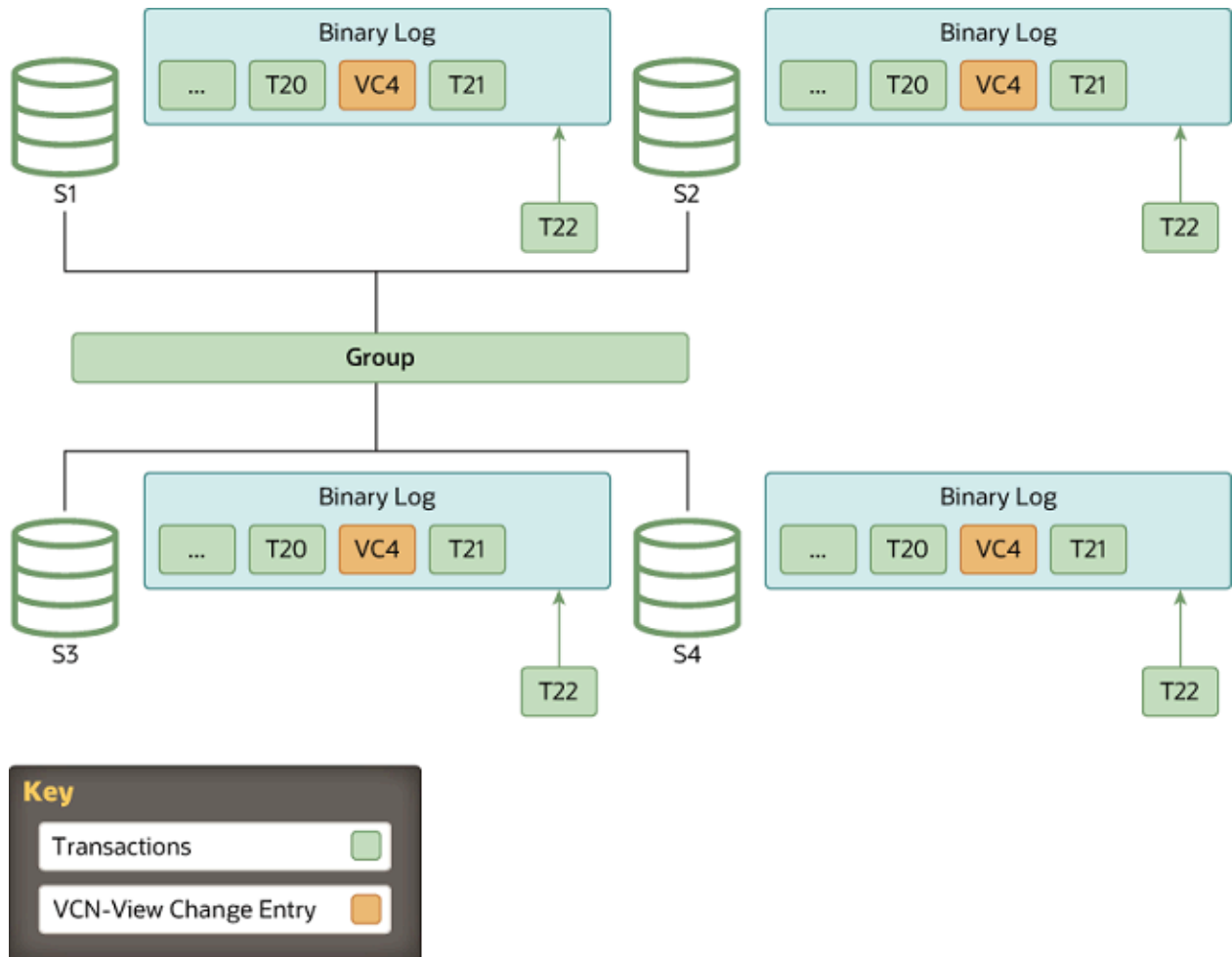
Figure 20.12 Instance Online
