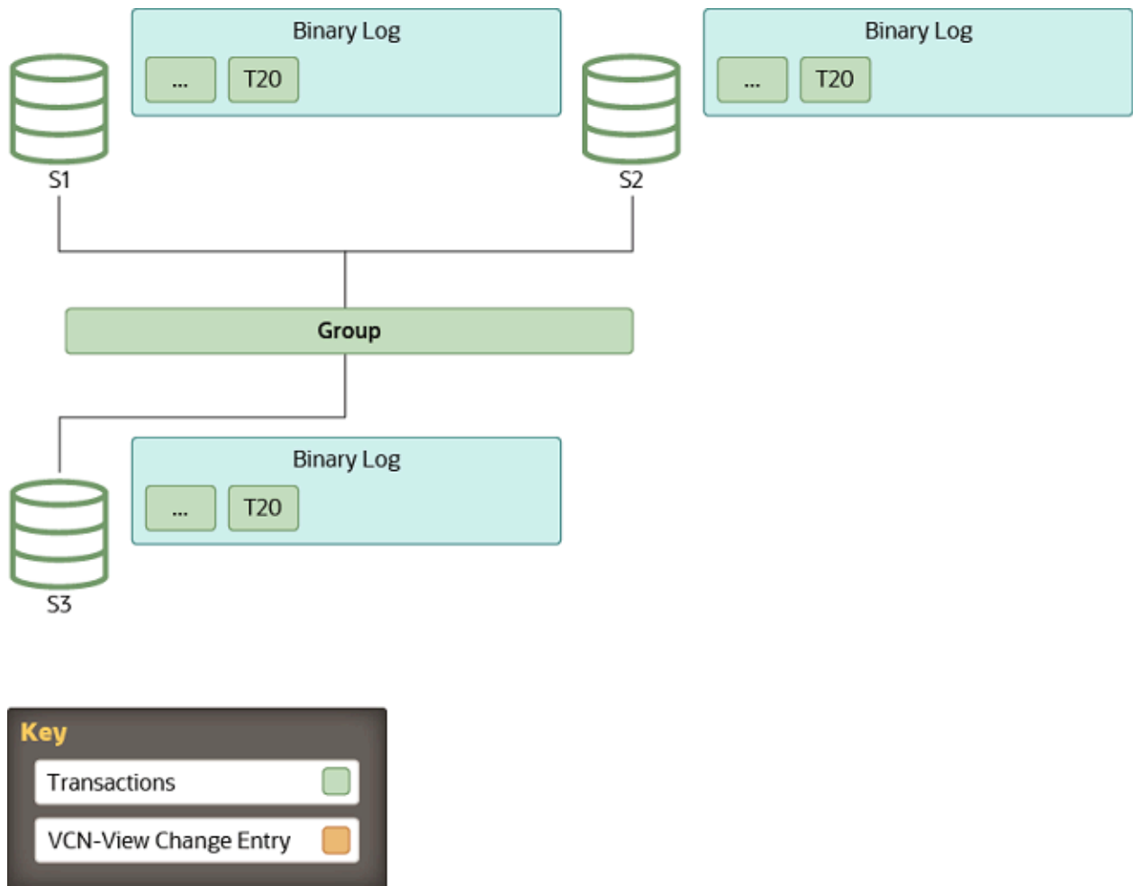
Figure 20.8 Stable Group
