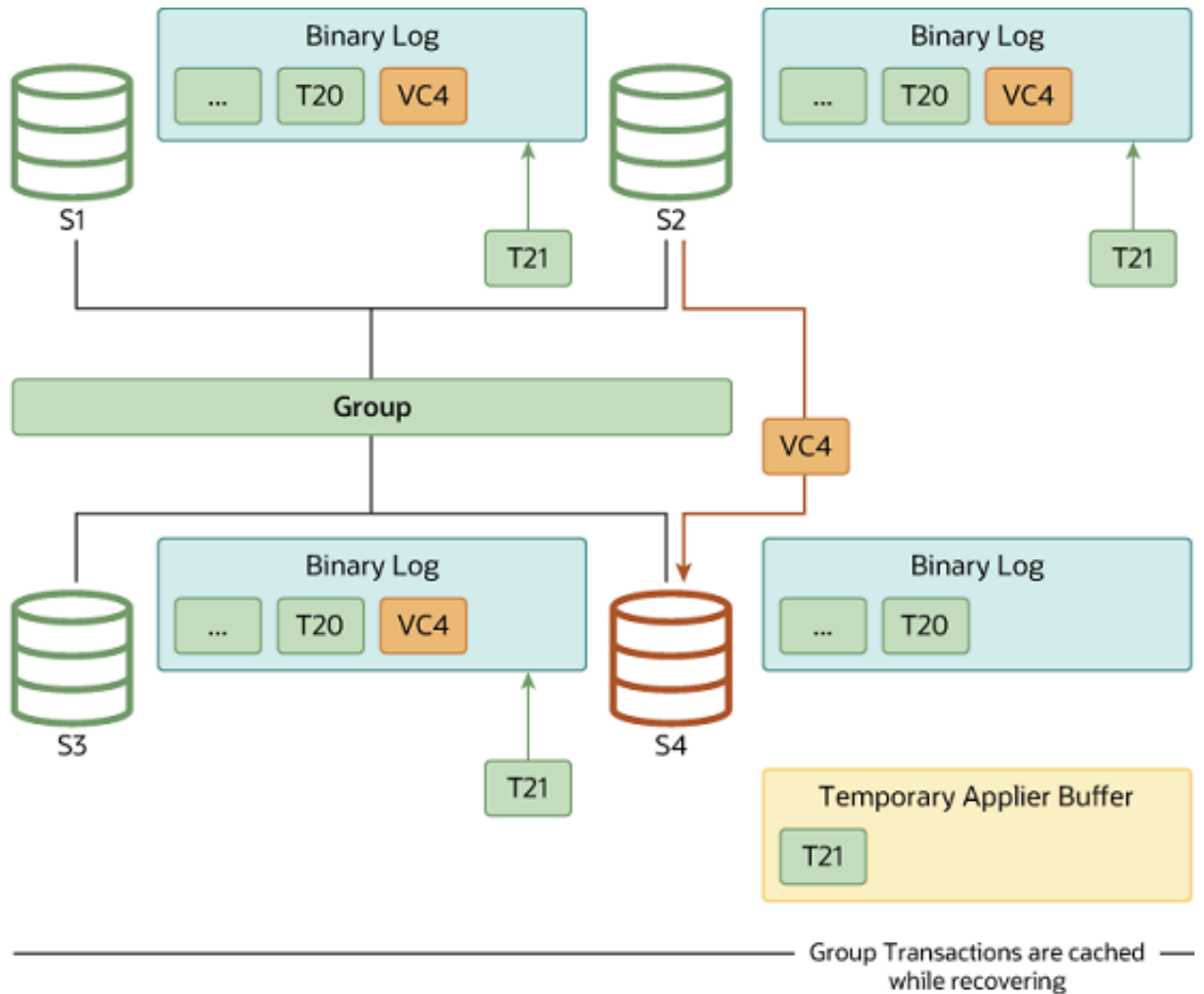
Figure 20.11 Queued Transactions
