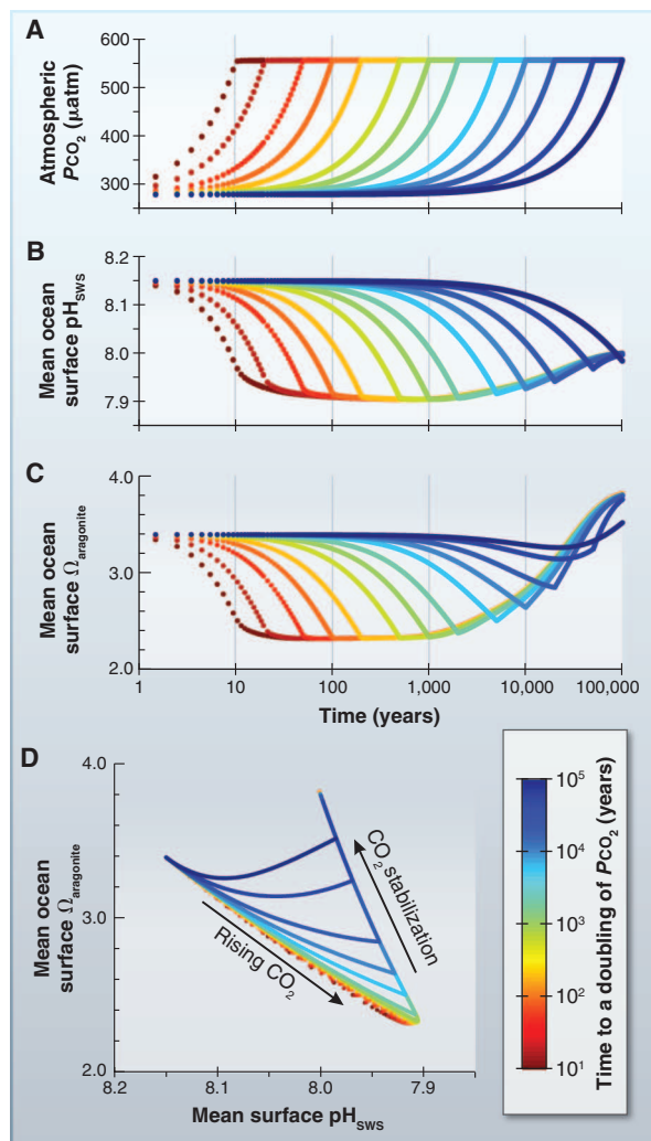
Fig. 3. The trajectories of mean ocean surface pH and aragonite saturation ( \Omega_{\text{aragonite}} ) become progressively decoupled as the rate of atmospheric P\text{CO}_2 change increases. The four panels show the results of a series of experiments in an Earth system model (2). (A) Prescribed linear increases of atmospheric P\text{CO}_2 (on a \log_{10} scale) from \times 1 to \times 2 preindustrial \text{CO}_2 , with the different model experiments spanning a range of time scales (but experiencing the same ultimate \text{CO}_2 change). (B) Evolution of mean surface pH in response to rising \text{CO}_2 . (C) Evolution of mean surface \Omega_{\text{aragonite}} . (D) A cross-plot illustrating how \Omega_{\text{aragonite}} is progressively decoupled from pH as the rate of P\text{CO}_2 increase slows, with future-relevant rate of P\text{CO}_2 increase showing a diagonal trajectory from top left to bottom right, whereas slow P\text{CO}_2 increases result in an almost horizontal trajectory toward lower pH with very little saturation change. All plots are color-coded from red (“fast”) to blue (“slow”). These model results include both climate and long-term (silicate) weathering feedback. See (2) and fig. S1 for the role of these and other feedbacks.
