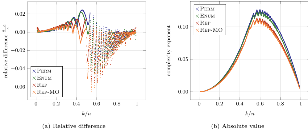
Fig. 8: Complexity exponents \tilde{c} for different regular-ISD variants after resolving rounding issues and relative difference to approximate exponents obtained in Sections 4.1 to 4.4.
