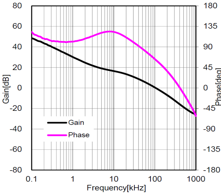
Figure 2. Frequency Characteristic (Datasheet)
