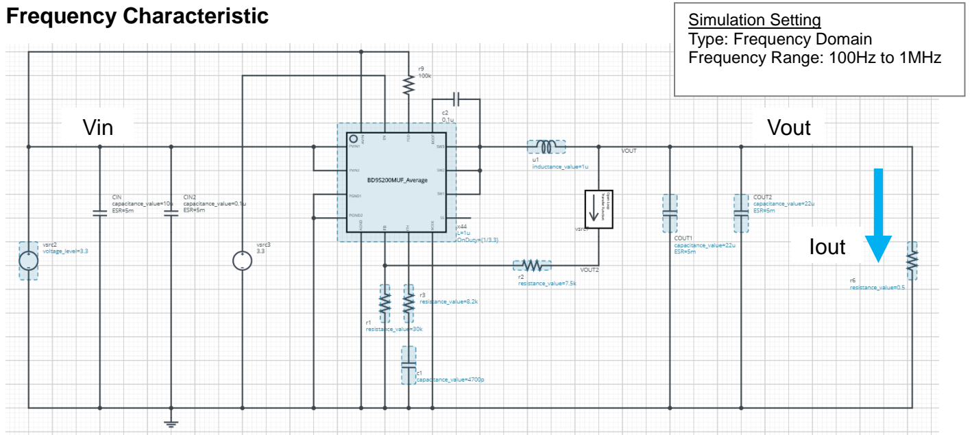
Figure 1. Simulation Schematic
