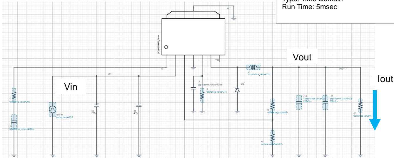
Figure 1. Simulation Schematic
