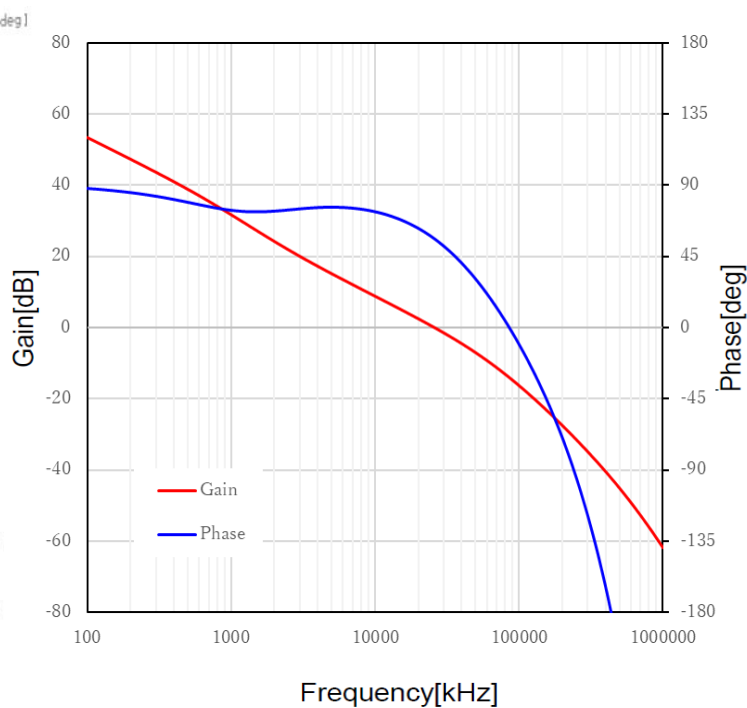
Figure 3. Frequency Characteristic (ROHM Solution Simulator)
