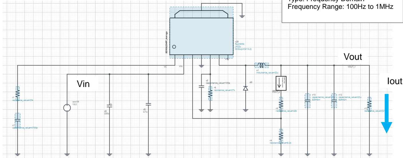
Figure 1. Simulation Schematic
