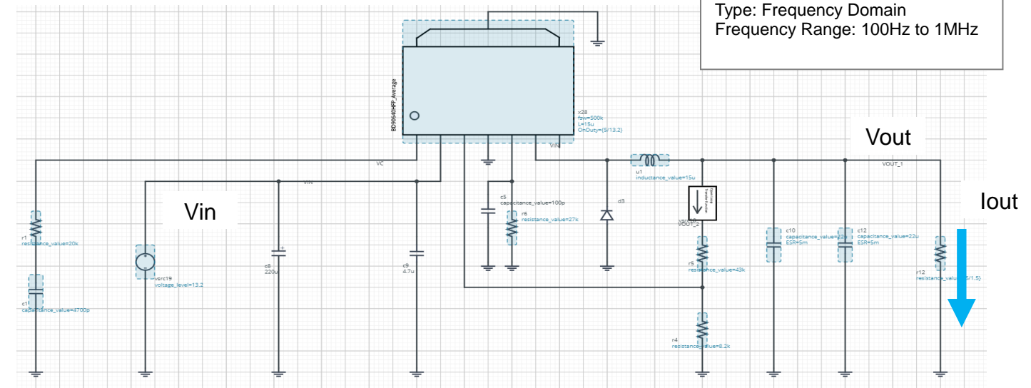
Figure 1. Simulation Schematic
