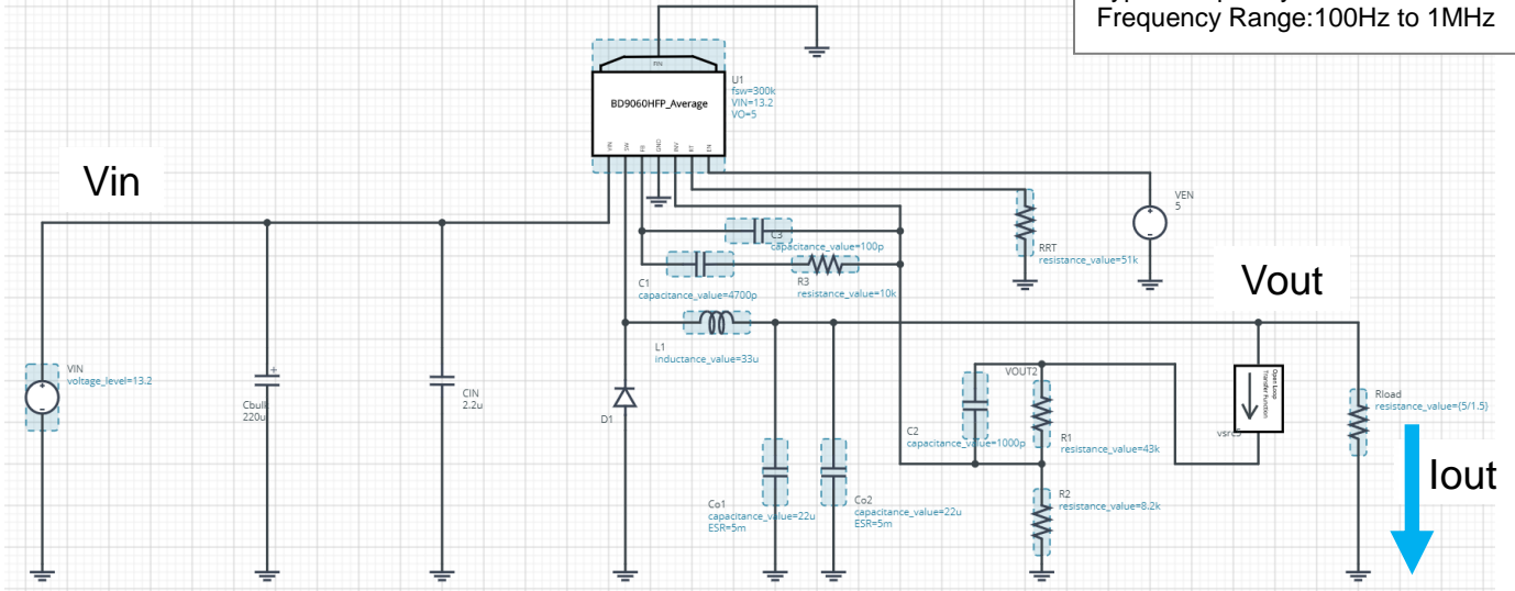
Figure 1. Simulation Schematic
