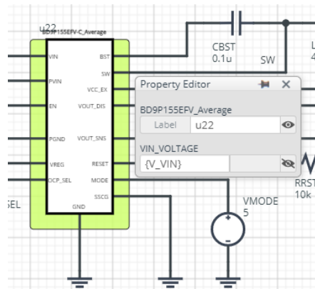
Figure 4. Property Editor of BD9P155EFV-C_Average model
