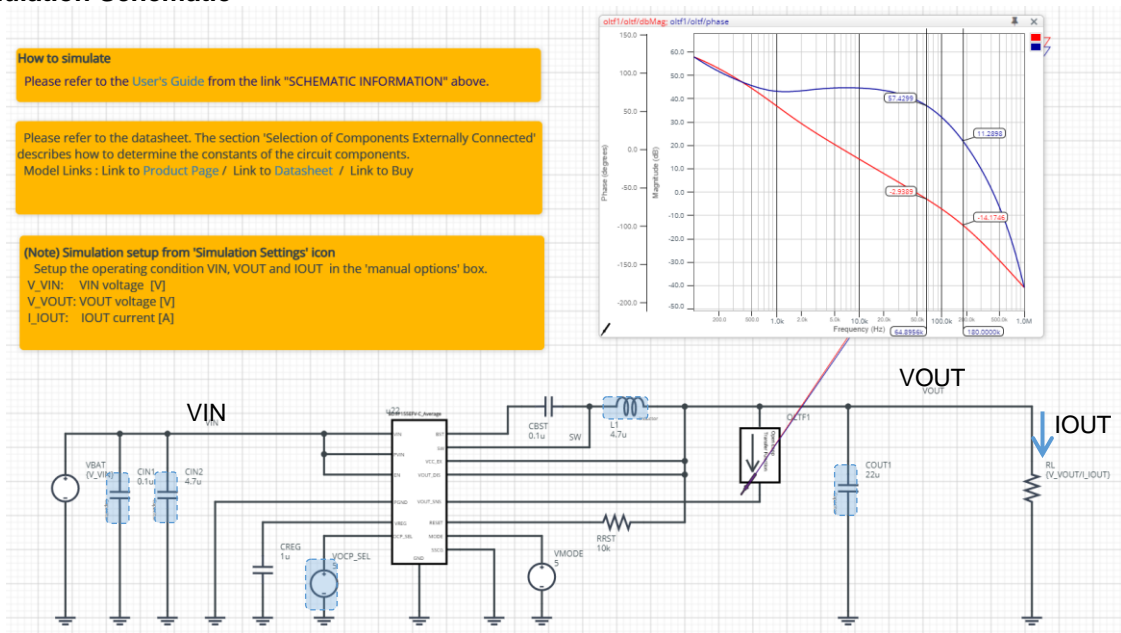
Figure 1. Simulation Circuit
