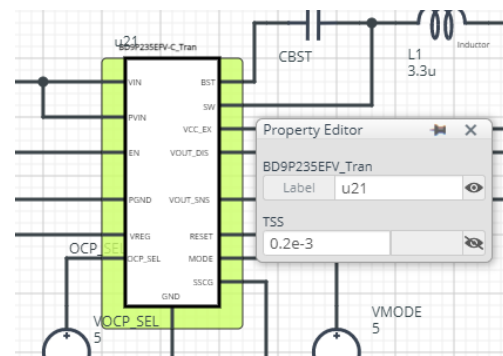
Figure 4. TSS property of BD9P235EFV-C_Tran
