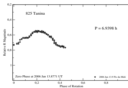
Fig. A.61. Composite lightcurve of 825 Tanina from its 2006 opposition.
