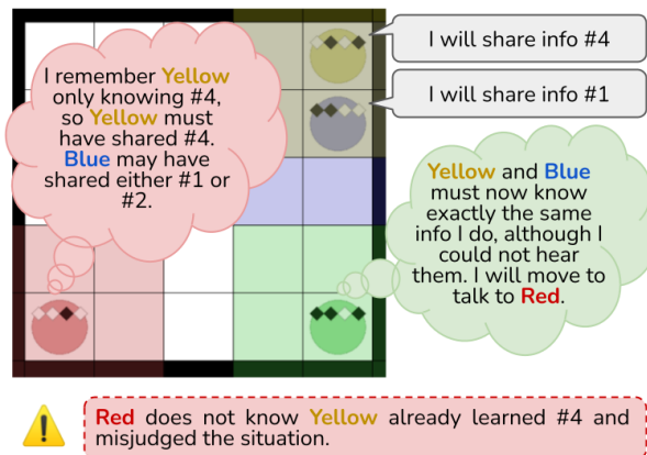
Figure 1. In SymmToM, agents aim to gain all available information (depicted as diamonds, black for known, white for unknown). Since hearing is limited to its neighbor cells, they must guess what happened beyond this range. Agents can see the whole grid, but mistakes in inferences may happen (as with the red agent).
