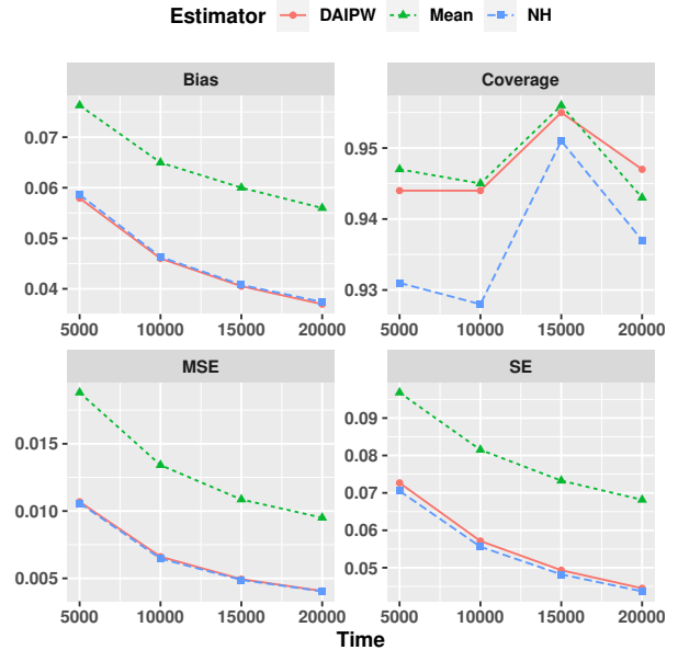
Figure 4. Evaluation of \epsilon -greedy with no finite delays
