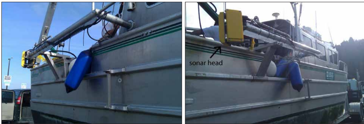
Figure 3. Fore and aft views of the SWATHplus sonar pole mount on the U.S. Geological Survey Pacific Coastal and Marine Science Center R/V Parke Snavelly .
