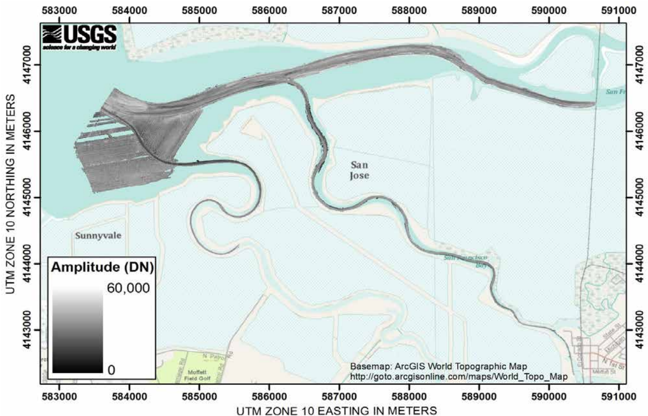
Figure 5. Map of backscatter amplitude (raw 16-bit digital number, DN), south San Francisco Bay,
