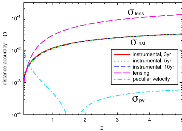
FIG. 10 (color online). Measurement accuracy of the luminosity distance with a single binary as a function of redshifts. The curves tagged \sigma_{\text{inst}} are those determined only by instrumental noise and with the observation time 3 yr (red, solid curve), 5 yr (green, dotted curve), and 10 yr (blue, short-dashed curve), respectively. The lensing error and the peculiar velocity error are represented by magenta (long-dashed) and light blue (dot-dashed) curves.
