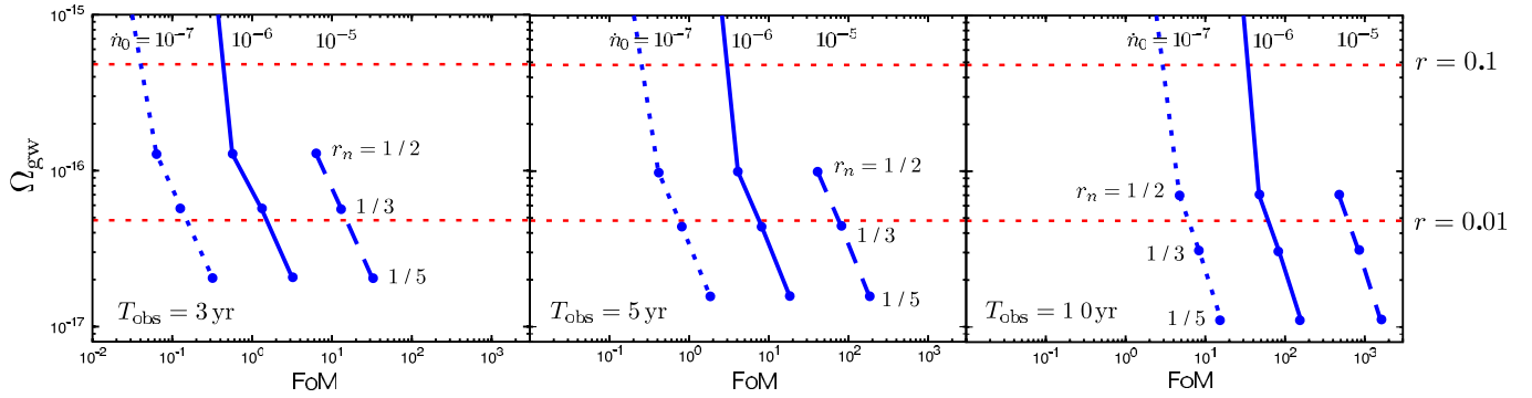
FIG. 9 (color online). FoM and \Omega_{\text{gw}} achievable with GW observation alone ( \eta = 0 ) for each parameter set of r_n , T_{\text{obs}} , and \dot{n}_0 . From the left to the right panels, the observation time is 3 yr, 5 yr, and 10 yr. In each panel, the merger rate is represented by curve types: \dot{n}_0 = 10^{-5} (dashed), 10^{-6} (solid), 10^{-7} (dotted), in the unit of \text{Mpc}^{-3} \text{yr}^{-1} . On each curve, points from the top to the bottom correspond to r_n = 1/2 , 1/3 , and 1/5 . The horizontal lines correspond to r = 0.1 and 0.01 at CMB scale in the de-Sitter inflation.
