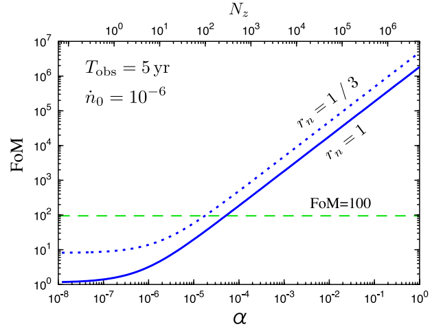
FIG. 7 (color online). FoM as a function of \alpha defined in Eq. (19) or N_z . The observation time and the merger rate are fixed to T_{\text{obs}} = 5 yr and \dot{n}_0 = 10^{-6} \text{Mpc}^{-3} \text{yr}^{-1} . The horizontal dashed line represents FoM = 100. The solid and dotted curves are the case with r_n = 1 and 1/3 , respectively.
