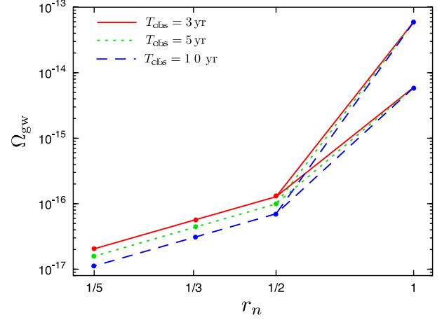
FIG. 8 (color online). \Omega_{\text{gw}} detectable with SNR = 5 for each parameter set of r_n , T_{\text{obs}} , and \dot{n}_0 . The observation time is denoted by colors: T_{\text{obs}} = 3 yr (red, solid), 5 yr (green, dotted), 10 yr (blue, dashed). For a fixed observation time, the merger rate only affects the r_n = 1 case: the upper and lower lines correspond to \dot{n}_0 = 10^{-6} , and 10^{-7} \text{ Mpc}^{-3} \text{ yr}^{-1} , respectively. For \dot{n}_0 = 10^{-5} case, no data is plotted due to the same reason in Table IV.
