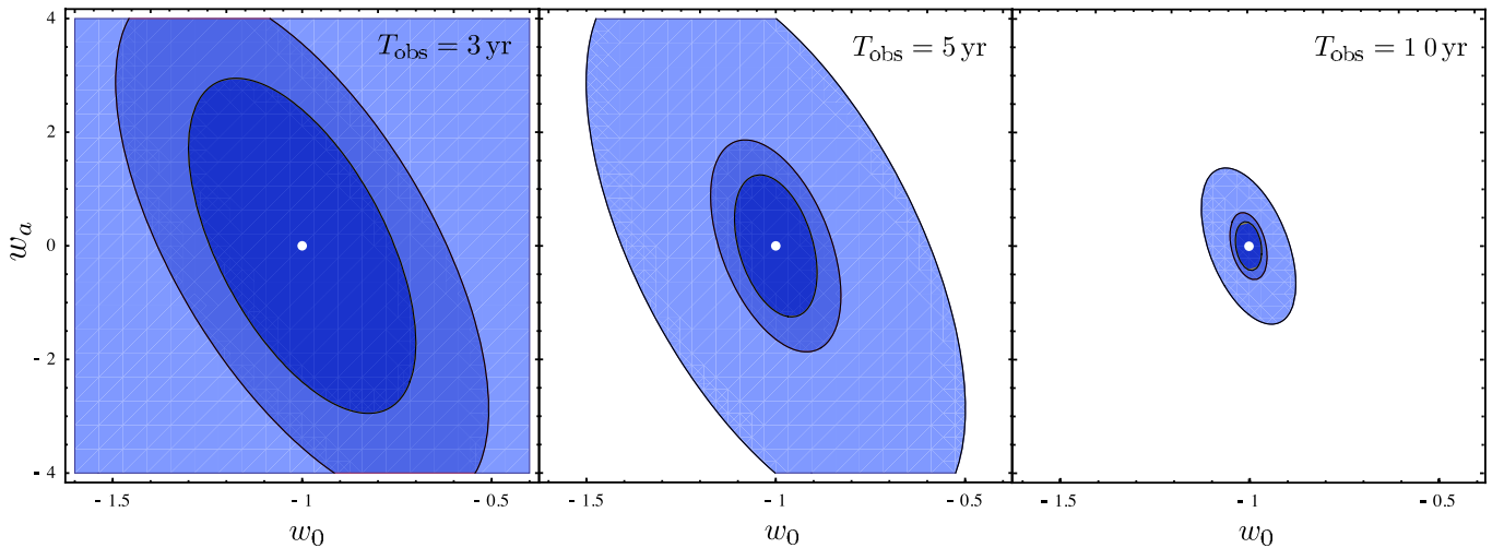
FIG. 4 (color online). w_0 — w_a error ellipses marginalized over \Omega_m . The merger rate is fixed to \dot{n}_0 = 10^{-6} \text{Mpc}^{-3} \text{yr}^{-1} . From the left to the right panels, the observation time is 3 yr, 5 yr, and 10 yr. In each panel, the larger to smaller ellipses denote those with r_n = 1 , 1/3, and 1/5, respectively. The dot at the center is our fiducial value: w_0 = -1 and w_a = 0 .
