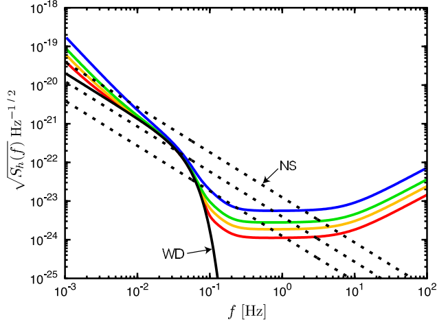
FIG. 1 (color online). Noise curves of default DECIGO (solid blue curve) and those scaled by r_n = 1/2 (green), 1/3 (orange), 1/5 (red), which include the confusion noise from a number of WD binaries. The WD-binary foreground \sqrt{S_h^{\text{WD}}} is shown with solid, black curve. The three diagonal lines represent the NS-binary foreground \sqrt{S_h^{\text{NS}}} before subtraction (or \mathcal{R}_{\text{NS}} = 1 ) with \dot{n}_0 = 10^{-5}, 10^{-6}, 10^{-7} Mpc ^{-3} yr ^{-1} from the top to the bottom.
