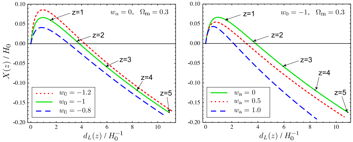
FIG. 3 (color online). d_L — X plot as a function of redshift. Left: w_0 is varied, while w_a and \Omega_m are fixed. Each curve corresponds to w_0 = -1.2 (red, dotted curve), w_0 = -1 (green, solid curve), w_0 = -0.8 (blue, dashed curve). Right: w_a is varied, while w_0 and \Omega_m are fixed. Each curve corresponds to w_a = 0 (green, solid curve), w_a = 0.5 (red, dotted curve), w_a = 1.0 (blue, dashed curve). The green solid curves in both figures are for \Lambda CDM universe. The points corresponding to z = 1, 2, 3, 4, 5 are shown on the curve.
