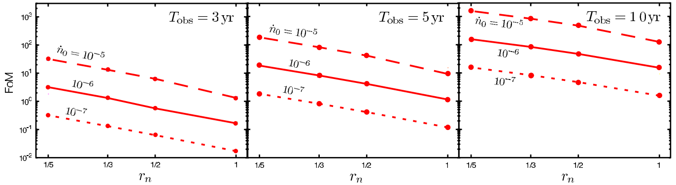
FIG. 5 (color online). FoM achievable for each parameter set of r_n , T_{\text{obs}} , and \dot{n}_0 . From the left to the right panels, the observation time is 3 yr, 5 yr, and 10 yr. In each panel, the merger rate is represented by curve types: \dot{n}_0 = 10^{-5} (dashed), 10^{-6} (solid), 10^{-7} (dotted), in the unit of \text{Mpc}^{-3} \text{yr}^{-1} .
