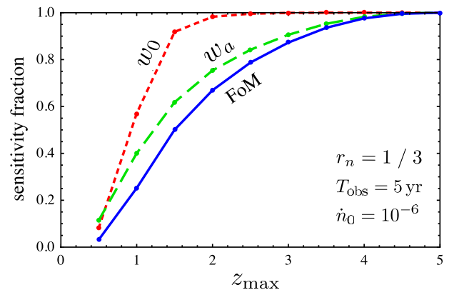
FIG. 6 (color online). Redshift dependence of the measurement accuracies in d_L — X measurement: \text{FoM}/\text{FoM}(z_{\text{max}} = 5) (blue, solid), \Delta w_0(z_{\text{max}} = 5)/\Delta w_0 (red, dotted), \Delta w_a(z_{\text{max}} = 5)/\Delta w_a (green, dashed). Parameters are fixed to r_n = 1/3 , T_{\text{obs}} = 5 yr, and \dot{n}_0 = 10^{-6} \text{Mpc}^{-3} \text{yr}^{-1} .
