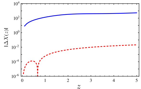
FIG. 11 (color online). Errors of X(z)/H_0 as a function of a redshift. The Solid curve denote the error due to instrumental noise in a GW observation, and the dotted curve denote the error propagating from the lensing error of d_L . Assumed parameters are r_n = 1 , T_{\text{obs}} = 3 yr, and \dot{n}_0 = 10^{-6} Mpc -3 yr -1 .
