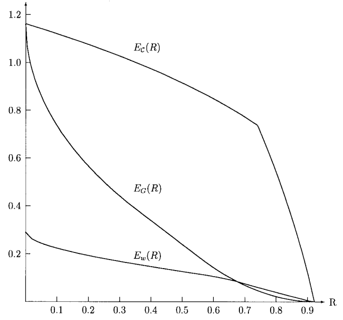
Fig. 5. Error exponents for block ( E_C^o(R) ), convolutional ( E_C(R) ), and woven convolutional ( E_w(R) ) codes.
