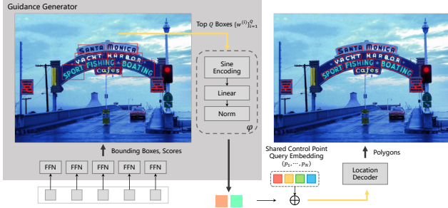
Figure 4. Illustration of the box-to-polygon detection process. The guidance generator predicts coarse bounding boxes and scores as shown in the left image. The coordinates of top Q boxes are fed to the differentiable encoding module \varphi and the encoded results are added to the shared control point query embeddings, which are taken by the location decoder for the final polygonal predictions.
