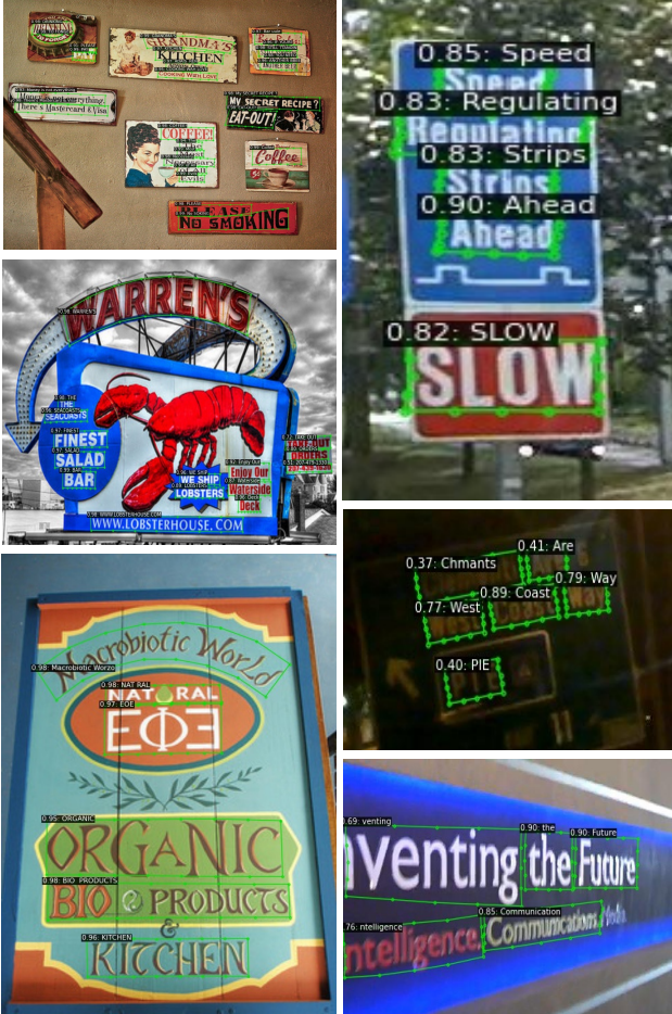
Figure 6. Qualitative results of TESTR on CTW1500 (left column) and ICDAR (right column) using polygonal annotations.
