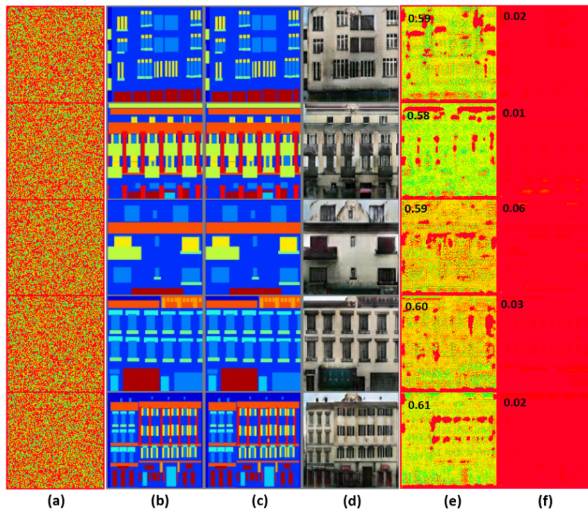
Figure 14. Visualization of samples used for GM Pix2Pix; (a) added template, (b) real images, (c) encrypted real images after adding a template, (d) manipulated images output by a GM, (e) recovered template from (c), and (f) recovered template from (d). Top left corner in last two columns shows the cosine similarity of the recovered template with the added template.
