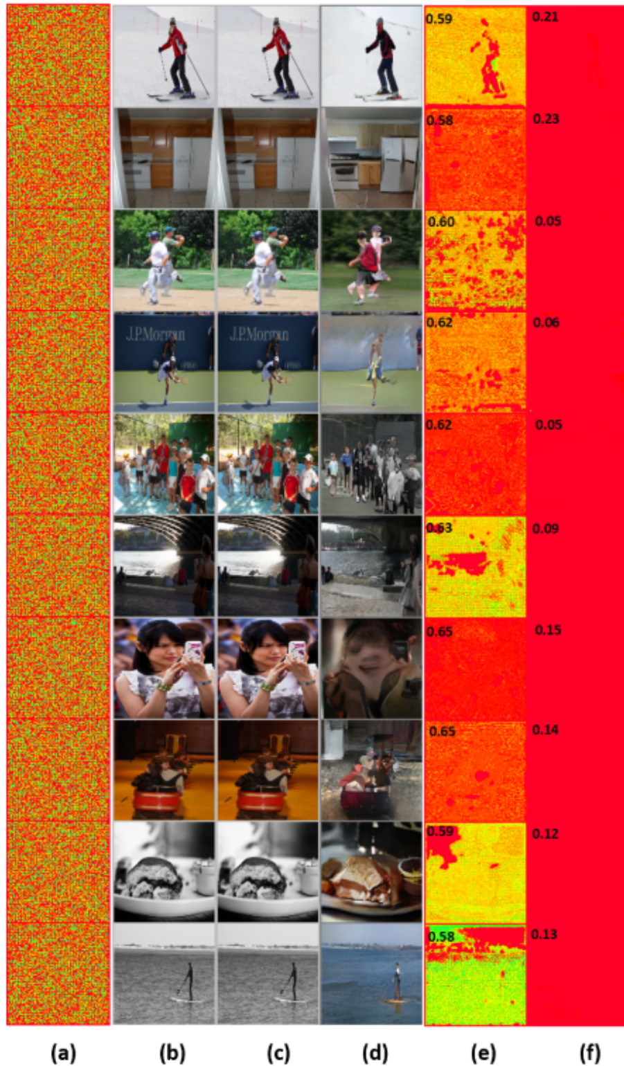
Figure 6. Visualization of samples used for GM GauGAN; (a) added template, (b) real images, (c) encrypted real images after adding a template, (d) manipulated images output by a GM, (e) recovered template from (c), and (f) recovered template from (d). Top left corner in last two columns shows the cosine similarity of the recovered template with the added template.
