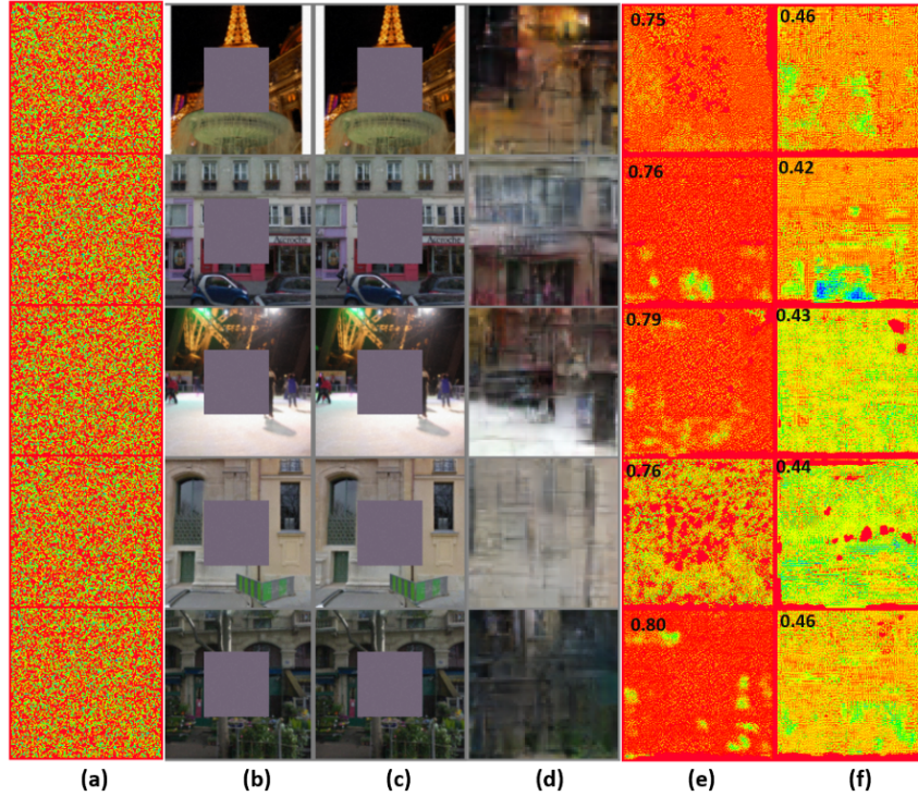
Figure 11. Visualization of samples used for GM CONT_Encoder; (a) added template, (b) real images, (c) encrypted real images after adding a template, (d) manipulated images output by a GM, (e) recovered template from (c), and (f) recovered template from (d). Top left corner in last two columns shows the cosine similarity of the recovered template with the added template.
