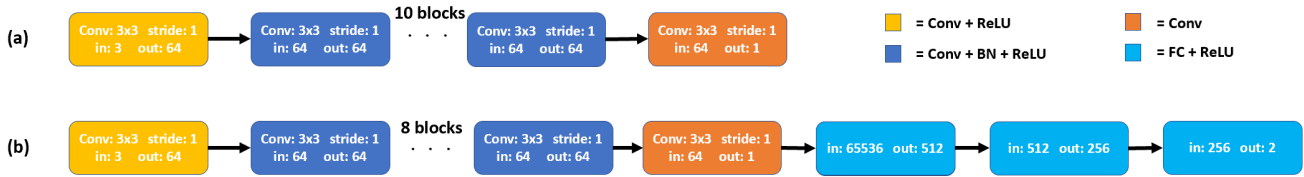
Figure 2. Network architecture for our (a) encoder (b) classifier network for image manipulation detection.
