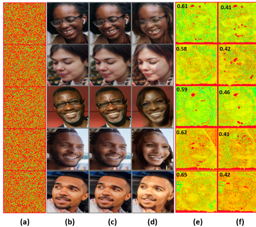
Figure 16. Visualization of samples used for GM CouncilGAN; (a) added template, (b) real images, (c) encrypted real images after adding a template, (d) manipulated images output by a GM, (e) recovered template from (c), and (f) recovered template from (d). Top left corner in last two columns shows the cosine similarity of the recovered template with the added template.
