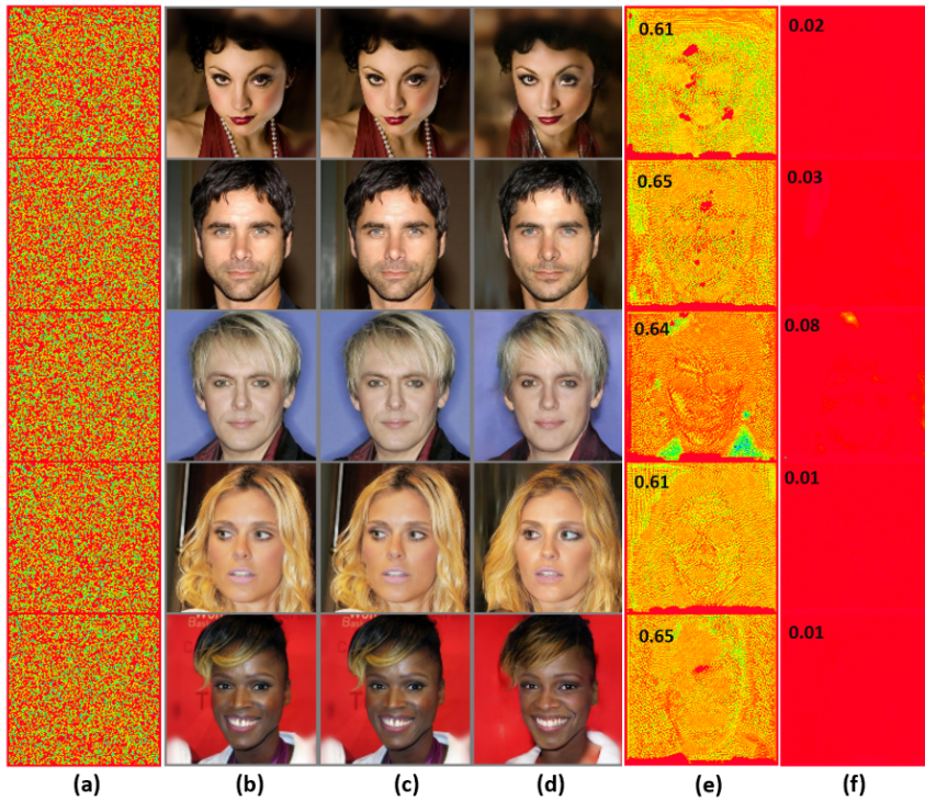
Figure 12. Visualization of samples used for GM SEAN; (a) added template, (b) real images, (c) encrypted real images after adding a template, (d) manipulated images output by a GM, (e) recovered template from (c), and (f) recovered template from (d). Top left corner in last two columns shows the cosine similarity of the recovered template with the added template.
