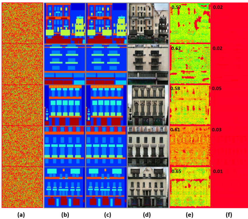
Figure 10. Visualization of samples used for GM BicycleGAN; (a) added template, (b) real images, (c) encrypted real images after adding a template, (d) manipulated images output by a GM, (e) recovered template from (c), and (f) recovered template from (d). Top left corner in last two columns shows the cosine similarity of the recovered template with the added template.
