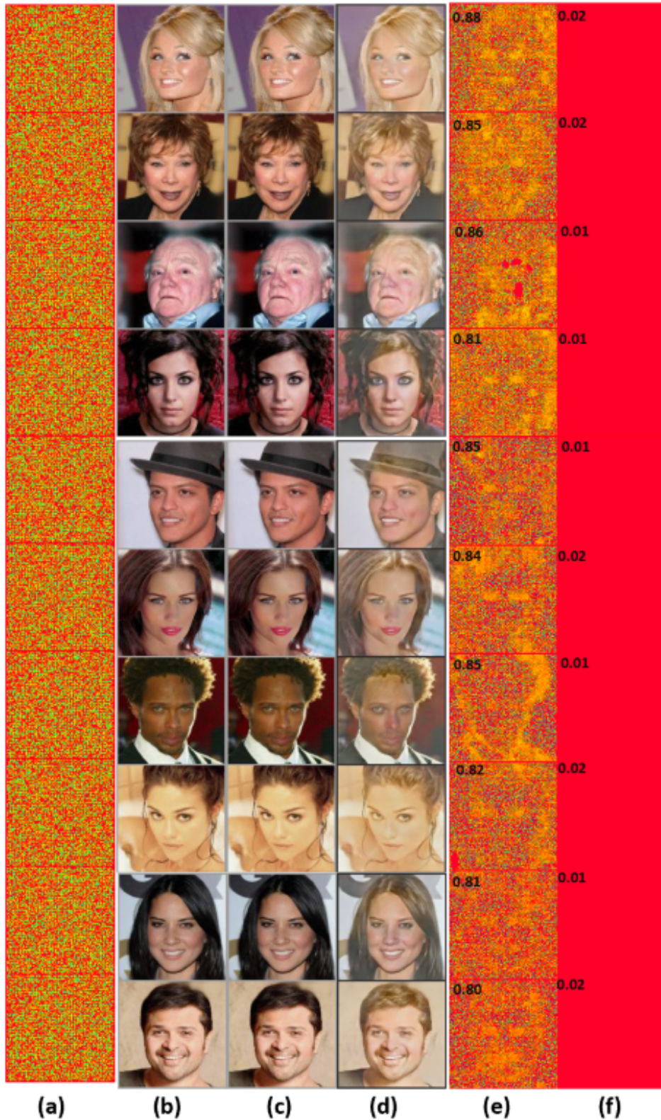
Figure 3. Visualization of samples used for GM STGAN; (a) added template, (b) real images, (c) encrypted real images after adding a template, (d) manipulated images output by a GM, (e) recovered template from (c), and (f) recovered template from (d). Top left corner in last two columns shows the cosine similarity of the recovered template with the added template.
