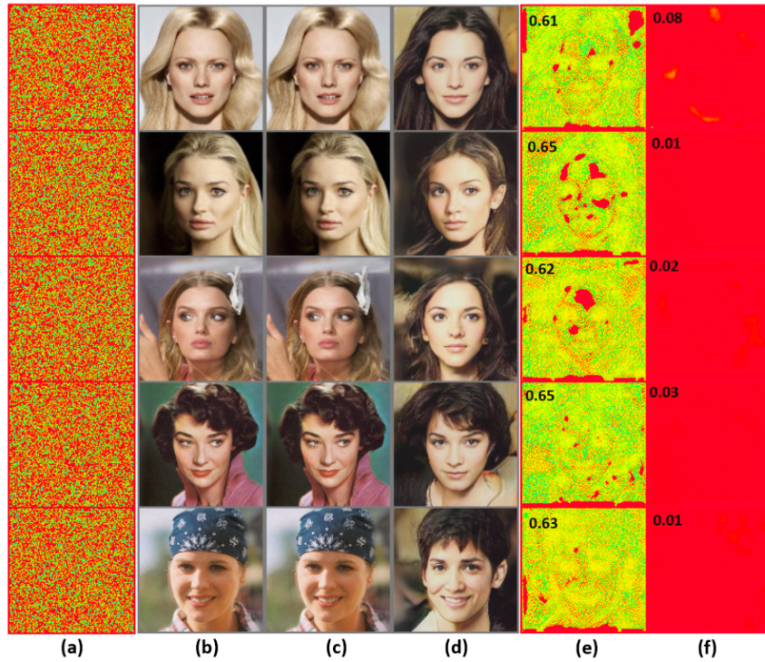
Figure 13. Visualization of samples used for GM ALAE; (a) added template, (b) real images, (c) encrypted real images after adding a template, (d) manipulated images output by a GM, (e) recovered template from (c), and (f) recovered template from (d). Top left corner in last two columns shows the cosine similarity of the recovered template with the added template.
