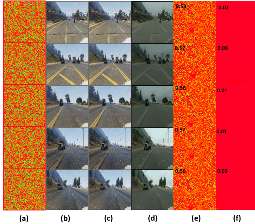
Figure 7. Visualization of samples used for GM UNIT; (a) added template, (b) real images, (c) encrypted real images after adding a template, (d) manipulated images output by a GM, (e) recovered template from (c), and (f) recovered template from (d). Top left corner in last two columns shows the cosine similarity of the recovered template with the added template.
