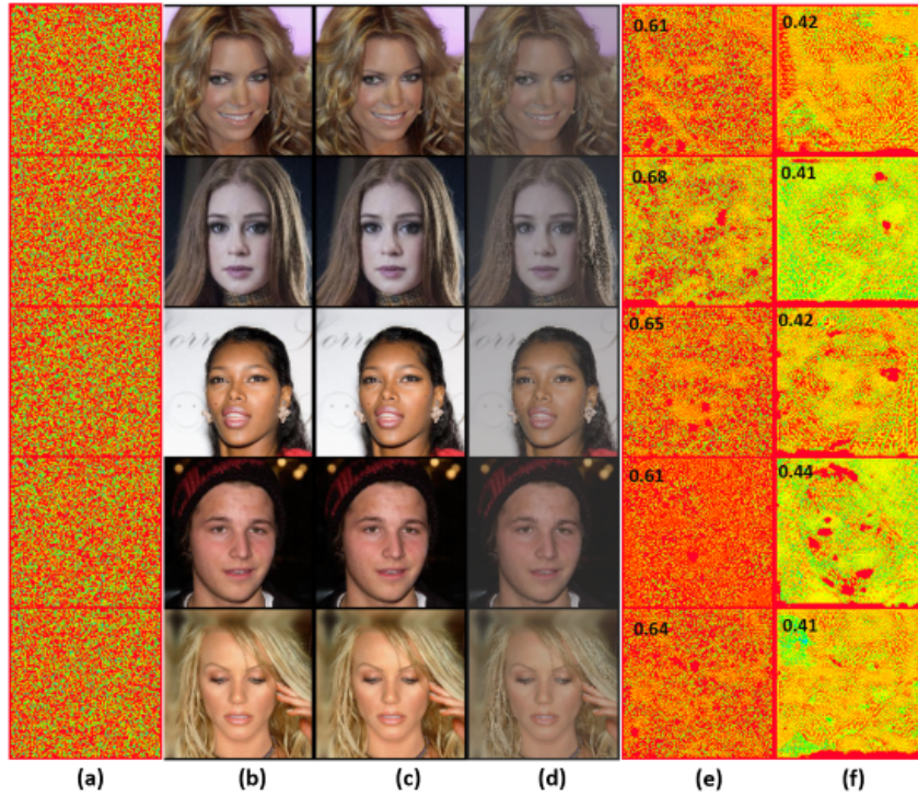
Figure 17. Visualization of samples used for GM ESRGAN; (a) added template, (b) real images, (c) encrypted real images after adding a template, (d) manipulated images output by a GM, (e) recovered template from (c), and (f) recovered template from (d). Top left corner in last two columns shows the cosine similarity of the recovered template with the added template.
