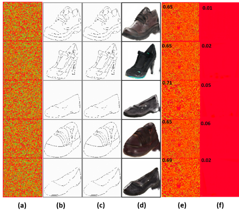
Figure 8. Visualization of samples used for GM MUNIT; (a) added template, (b) real images, (c) encrypted real images after adding a template, (d) manipulated images output by a GM, (e) recovered template from (c), and (f) recovered template from (d). Top left corner in last two columns shows the cosine similarity of the recovered template with the added template.
