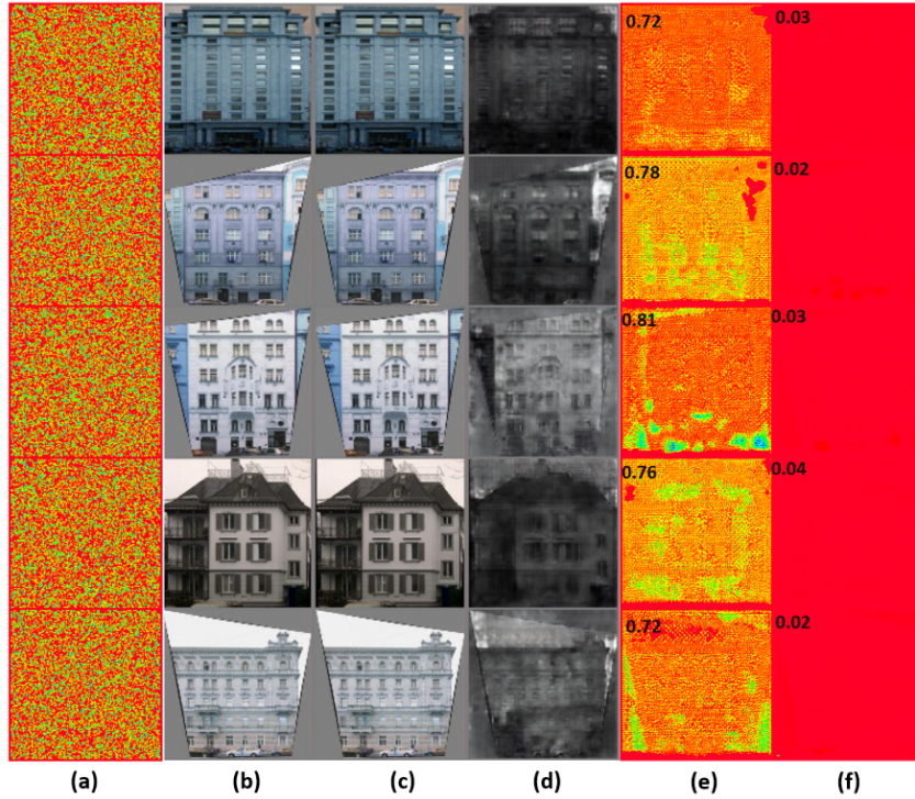
Figure 15. Visualization of samples used for GM DualGAN; (a) added template, (b) real images, (c) encrypted real images after adding a template, (d) manipulated images output by a GM, (e) recovered template from (c), and (f) recovered template from (d). Top left corner in last two columns shows the cosine similarity of the recovered template with the added template.
