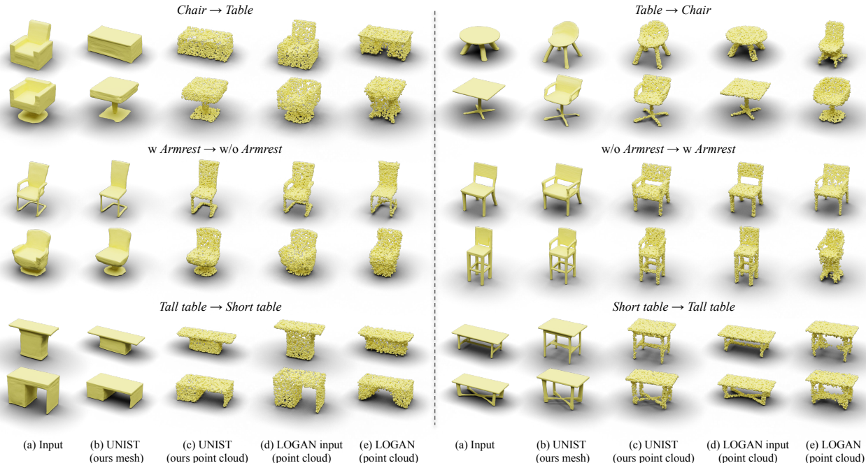
Figure 8. Comparison of translation results by UNIST (ours) and LOGAN on different 3D shapes. Row 1-2 (left): Chair \rightarrow Table (right): Table \rightarrow Chair . Row 3-4 (left): w Armrest \rightarrow w/o Armrest (right): w/o Armrest \rightarrow w Armrest . Row 5-6 (left): Tall table \rightarrow Short table , (right): Short table \rightarrow Tall table . (a) Test input mesh from voxel. (b) Translation by UNIST (ours) in mesh representation. (c) Translation by UNIST (ours) in point cloud representation. (d) LOGAN test input point cloud. (e) Translation by LOGAN.
