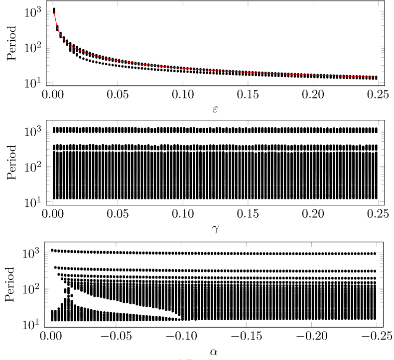
Figure 6. Parameters' influence on period of AP in FHN. Red curve in first sub-figure is the fitted curve : \text{Period} = 3.065 \times \varepsilon_{\alpha,\gamma}^{-0.8275} + 4.397 . ( discontinuity in third sub-figure means no valid AP generated. )
